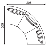
Banana 3-seat 90° top view
