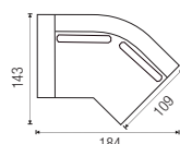
45 corner small arm L top view
